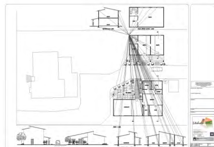
Plans for the new Woza Moya Centre
